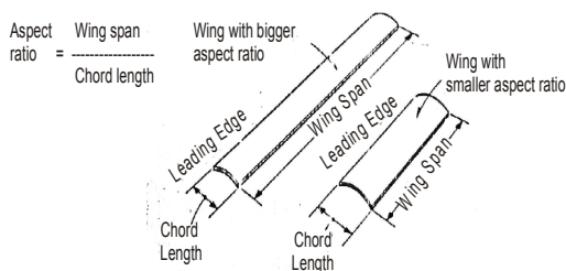
Fig 7 : Aspect Ratio
