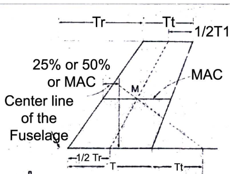
Fig 15 How to find Mean Aerodynamic Chord Mac
