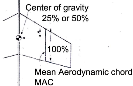
Fig 16 : Center of gravity is decided using MAC formula for any wing shape not rectangular
