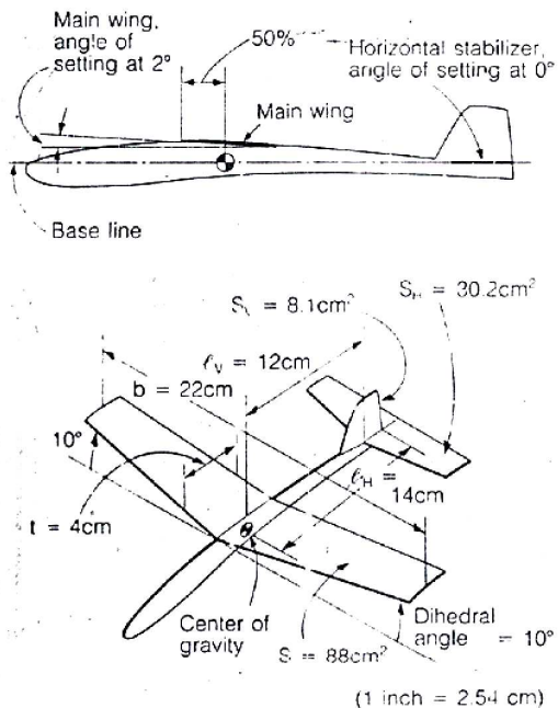
Fig.21 Test design for long duration flight
