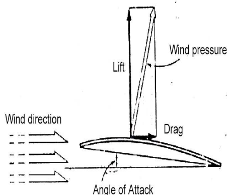
Fig.3 Angle of attack and forces on wing
