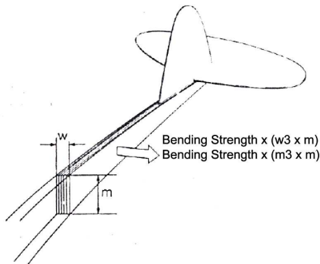
Fig 25 : Dimensions of the fuselage and bending strength
