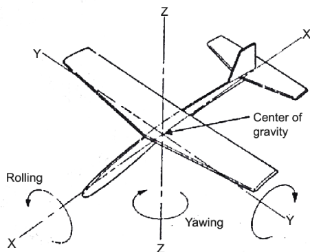
Fig 9 Inflight motion
