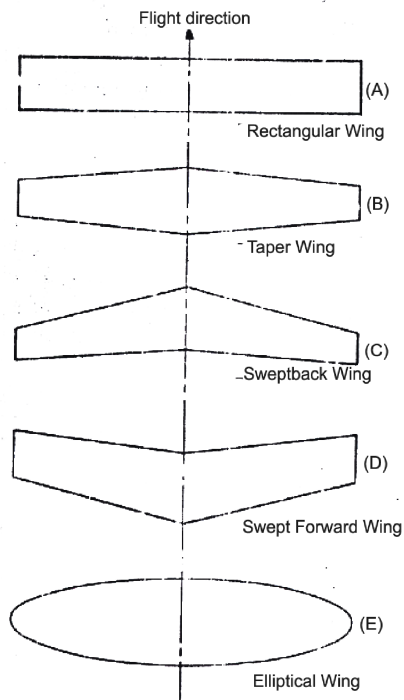
Fig 10 Wing Shapes
